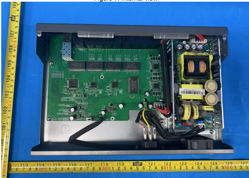
Figure 8. Internal view
