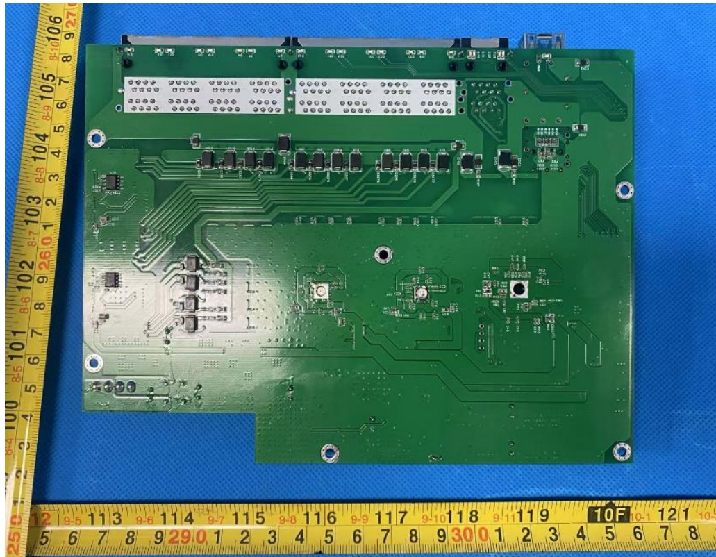
Figure 11. PCB view
